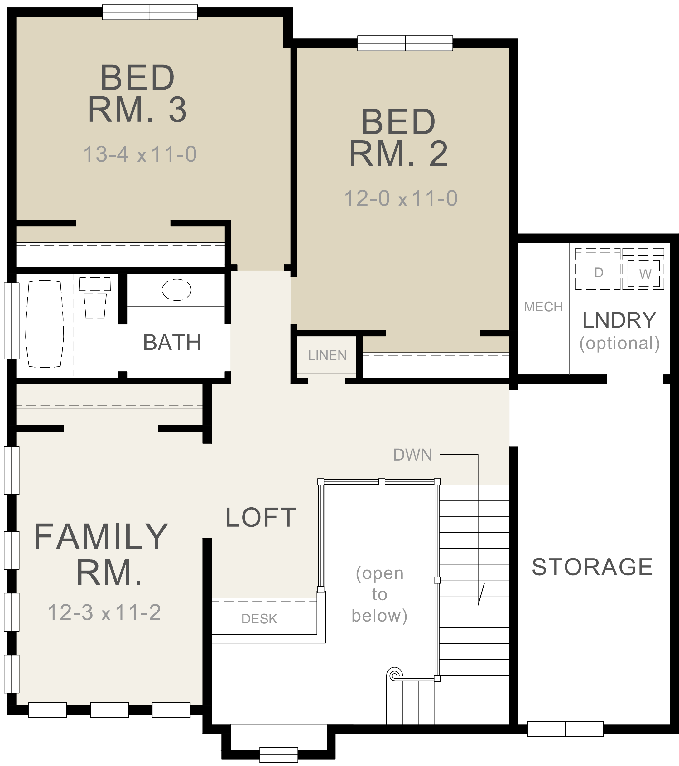
2ND FLOOR
