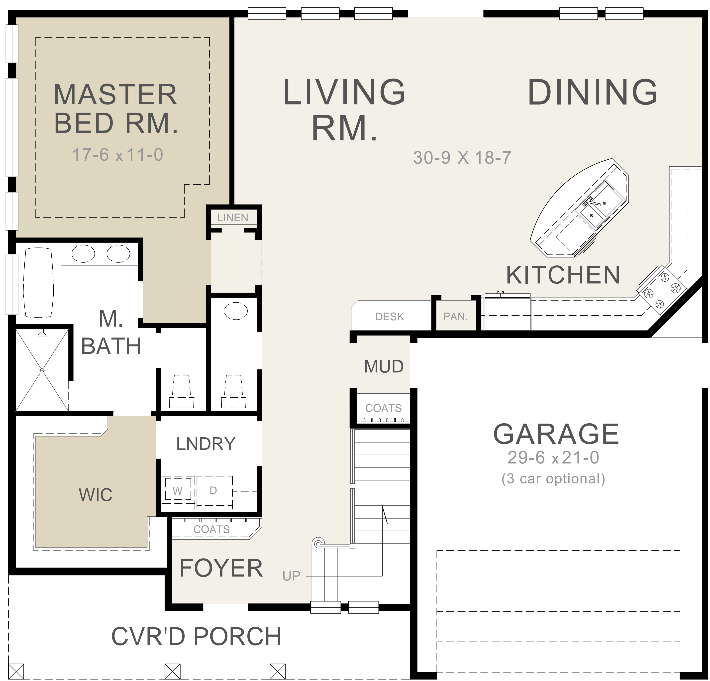
MAIN FLOOR
